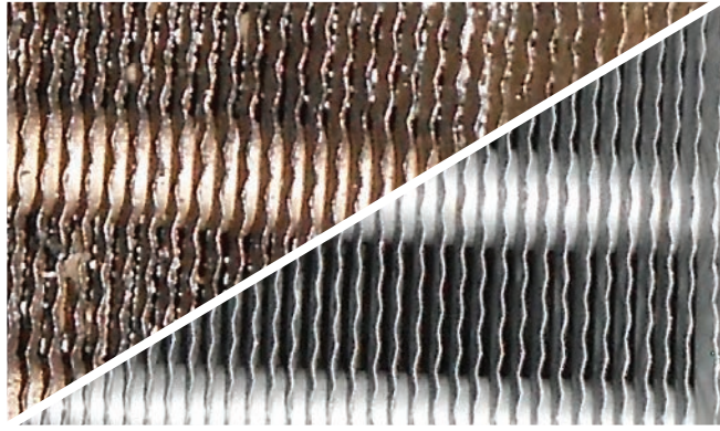
Coil After PURE-Steam
